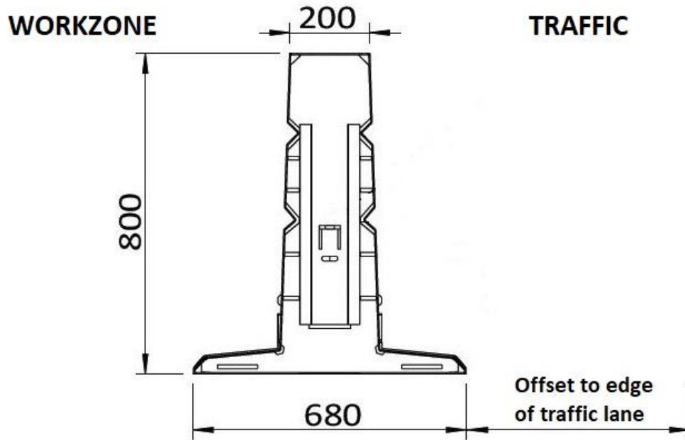
Typical cross section of Defender 100HC
