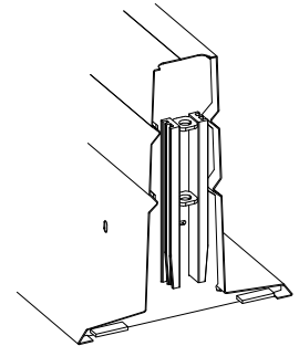
MALE END - 3D VIEW
