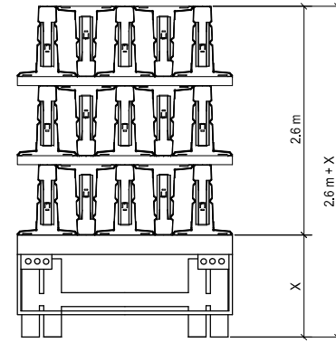
FULL TRUCK LOAD DETAIL USING 102 x 102 NOMINAL (89x89 ACTUAL) STEEL DUNNAGE
