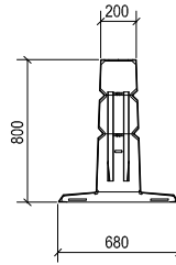
A - A MALE END
