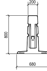
B - B FEMALE END
