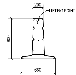
C - C LIFTING PLATE
